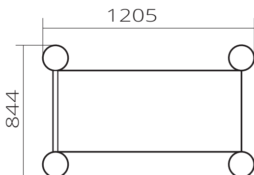
Foundation
